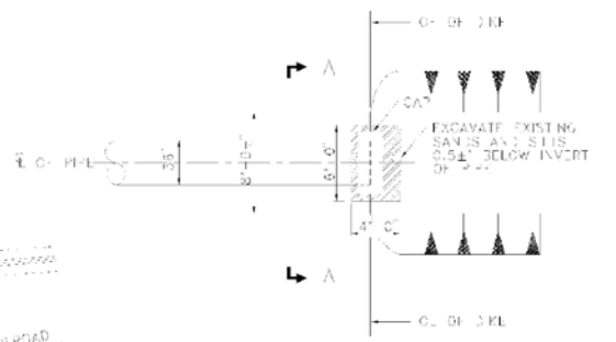
PLAN-DISC ARGUMENT PIPE JOINT
