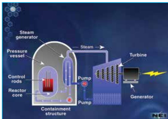
Typical Pressurized Water Reactor (PWR) Design
