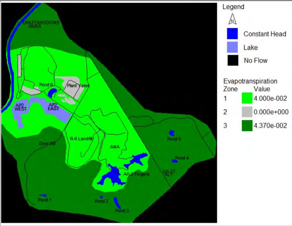
Figure 4-5 Evapotranspiration Zones – Layer 1
