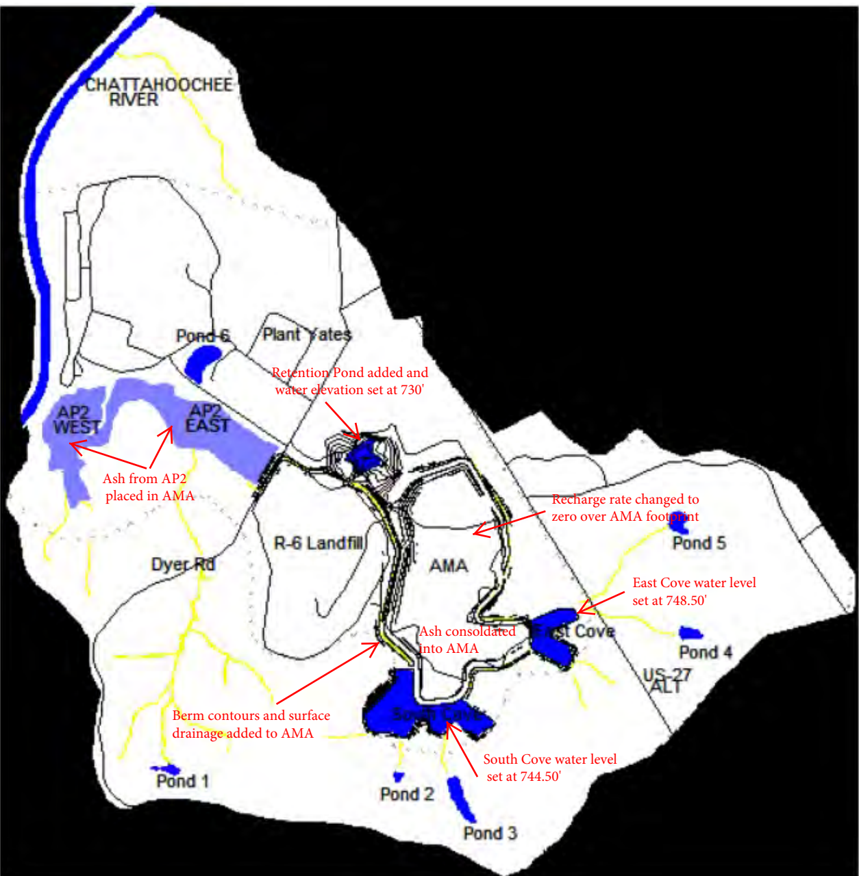
POST-CLOSURE MODEL CONFIGURATION
