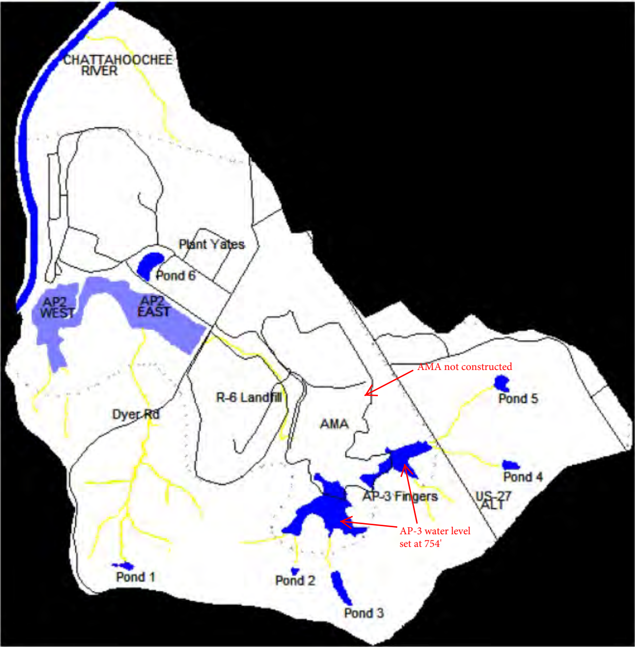
PRE-CLOSURE MODEL CONFIGURATION
